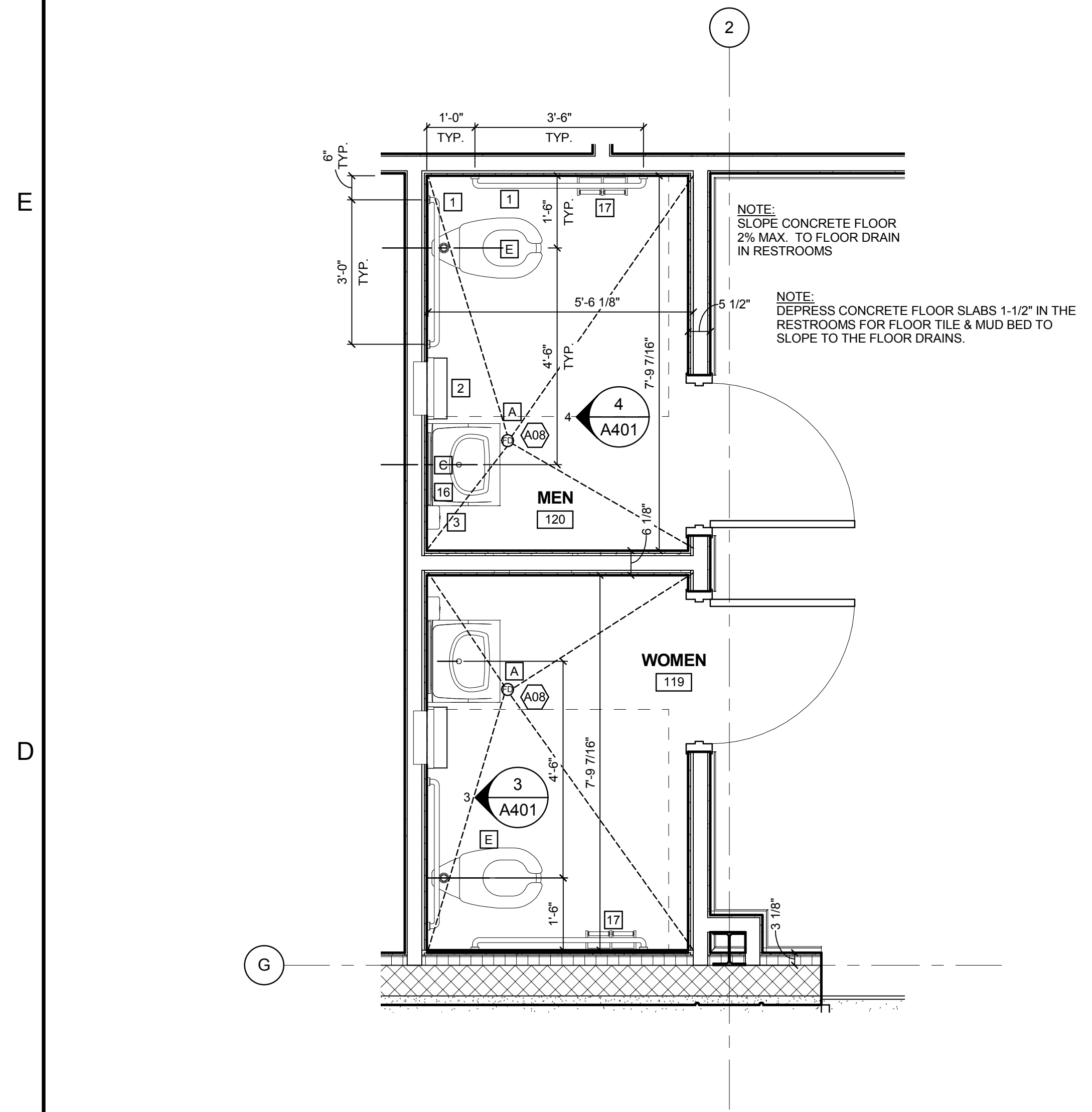
2 ENLARGED VISITOR'S RESTROOMS PLAN SCALE: 1/2" = 1'-0"
