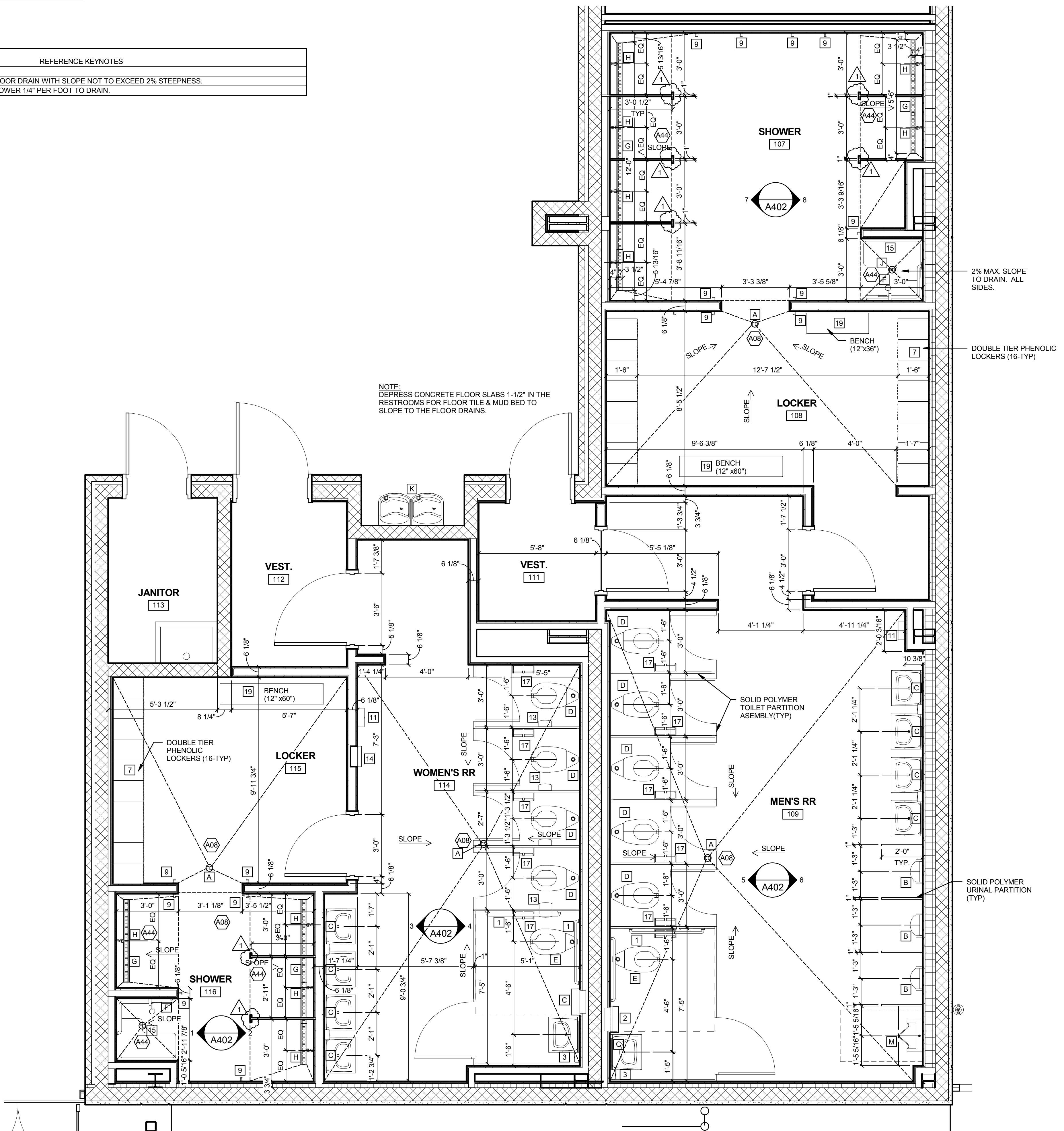
1 ENLARGED RESTROOM PLAN SCALE: 3/8" = 1'-0"
