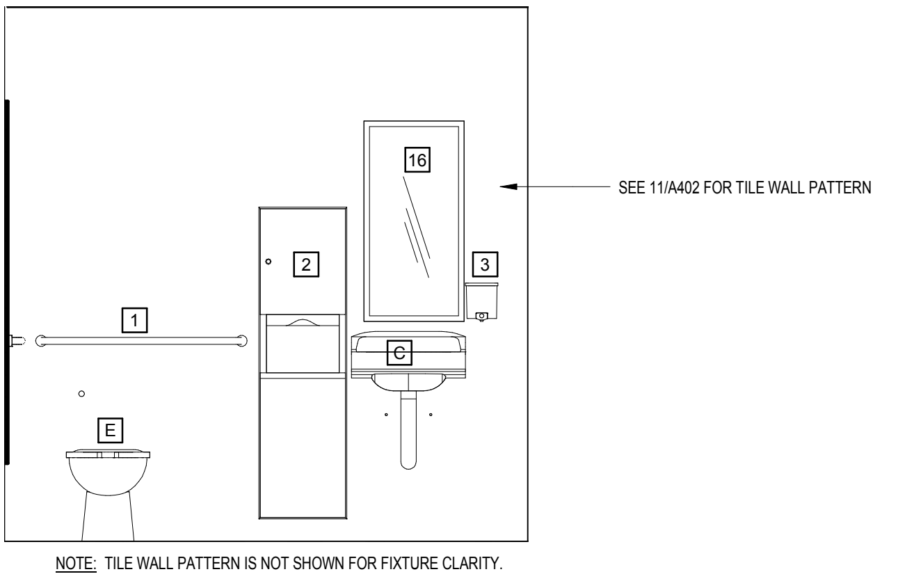
3 WOMEN'S RR-119 WEST ELEV. SCALE: 1/2" = 1'-0"
