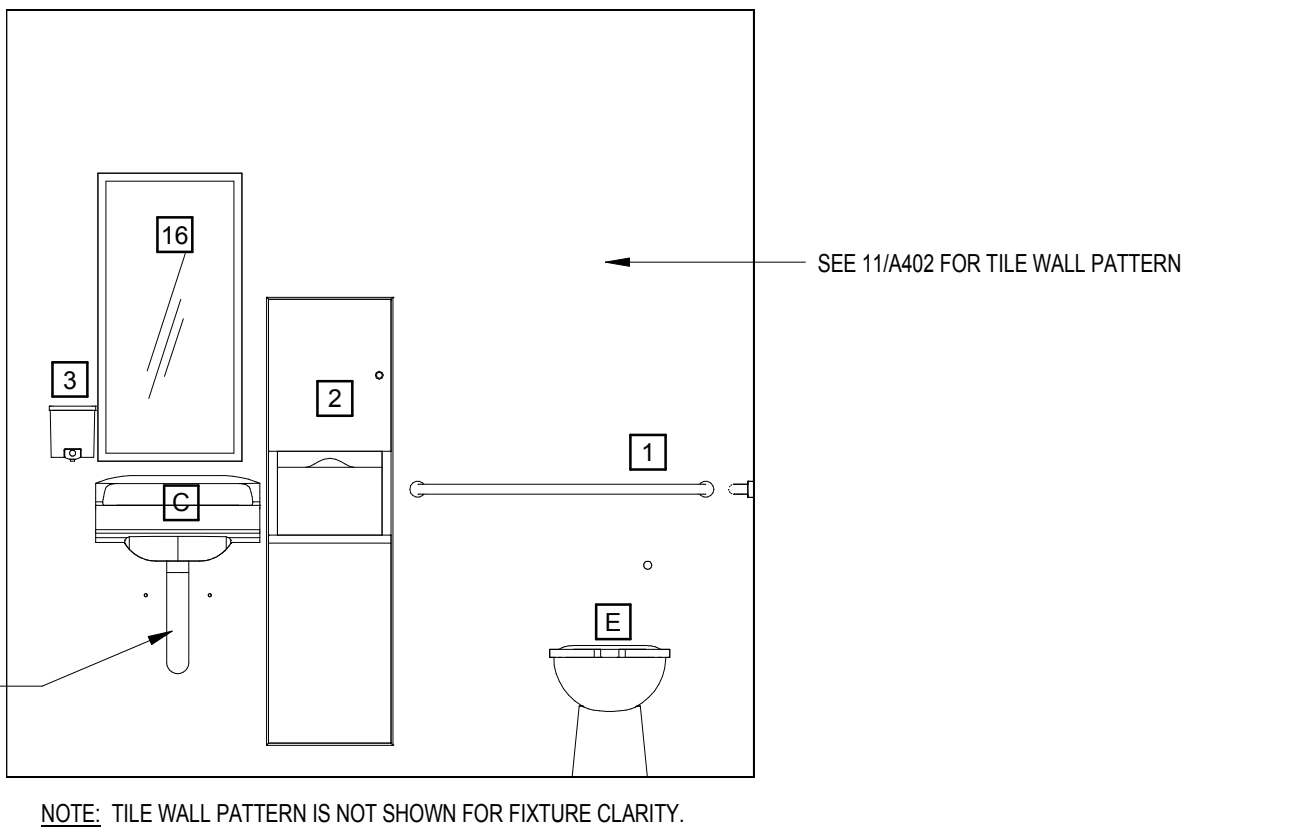
4 MEN'S RR-120 WEST ELEV. SCALE: 1/2" = 1'-0"
